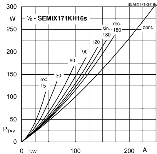
Fig. 1L: Power dissipation per thyristor/diode vs. on-state current
