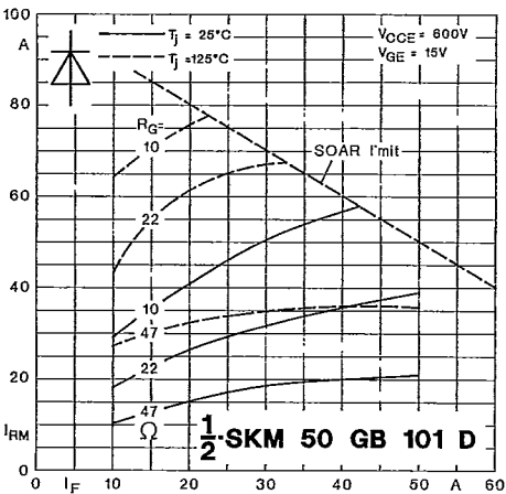
Fig. 40 a Diode peak reverse recovery current ( I_{RRM} )
