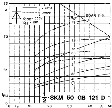
Fig. 40 b Diode peak reverse recovery current ( I_{RRM} )
