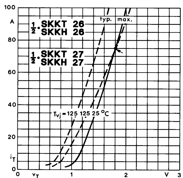
Fig. 8 On-state characteristics
