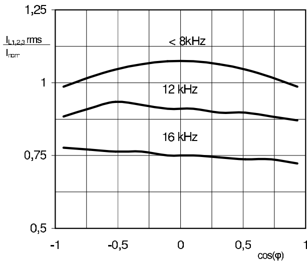
Fig. 1: Normalized output current vs. \cos(\varphi)
