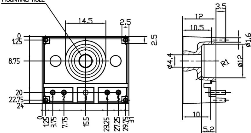
Case T 1 (Suggested hole diameter in the PCB for solder pins and mounting pins : 2mm)
